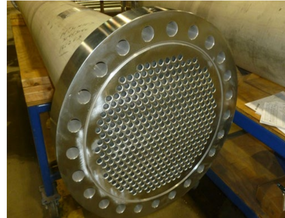
Fixed Tubesheet
