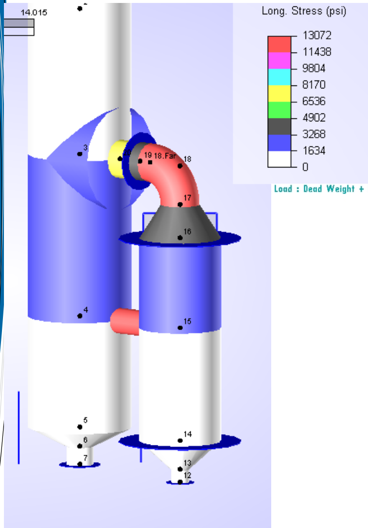
Column & Reboiler
