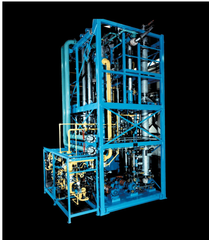
Multi-Stage Evaporator / Stripper TCE Removal
